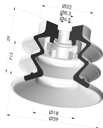
Sauggreifer 2.5 Falten Serie 96C Ø 40MM
