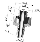
Separable Male Fitting M8
