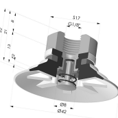
Flat Suction Cup Series 90, Ø 40 mm
