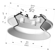
Bellows Suction Cup 1.5 folds Series 91, Ø 150 mm
