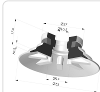
Flat Suction Cup Series 90, Ø 50 mm
