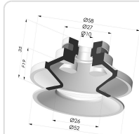
Bellows Suction Cup 1.5 folds Series 91, Ø 50 mm
